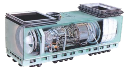
30.2 MW marine gas turbine module
