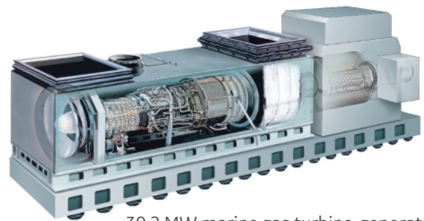
30.2 MW marine gas turbine-generator set
